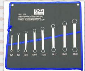
8 pce Double Ring Spanner set, extra flat 6x7, 8x9, 12x13, 14x15, 16x17, 18x19, 20x22mm
